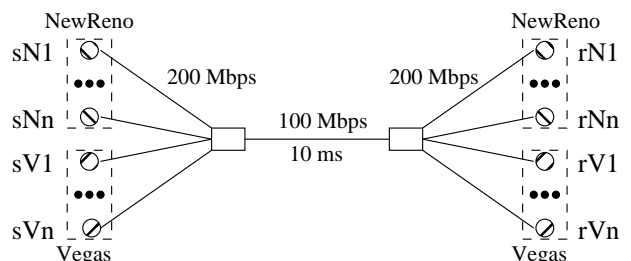
Fig. 3. Dumbbell topology
