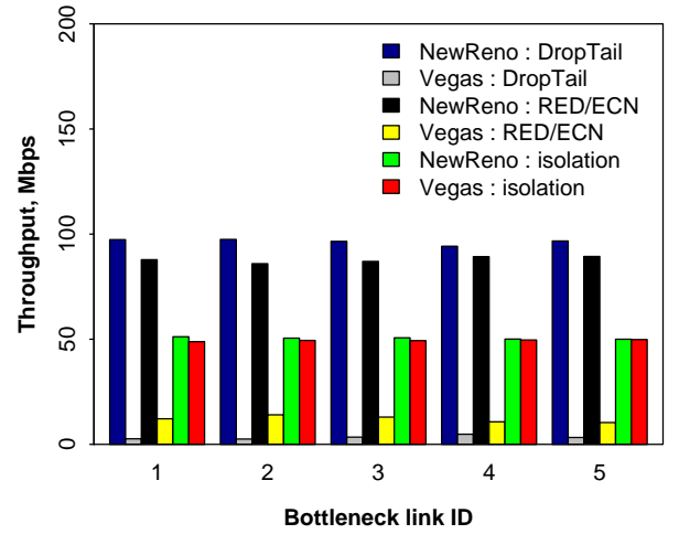
Fig. 12. Multi-bottleneck link topology. The average throughputs of TCP NewReno and TCP Vegas for different link serving schemes.
