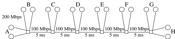
Fig. 11. Parking-lot topology
